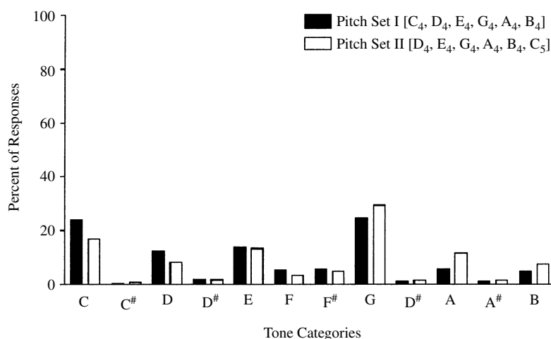
FIG 2. The average final-tone profile for nonmusicians in Experiment 2.
