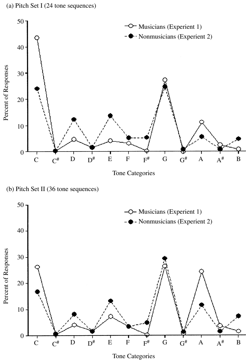
FIG 3. The distribution of responses of musicians and nonmusicians for the 60 tone sequences.
