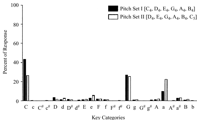
FIG 1. The average key profile for musicians in Experiment 1. Capital letters and small letters denote major and minor keys, respectively.
