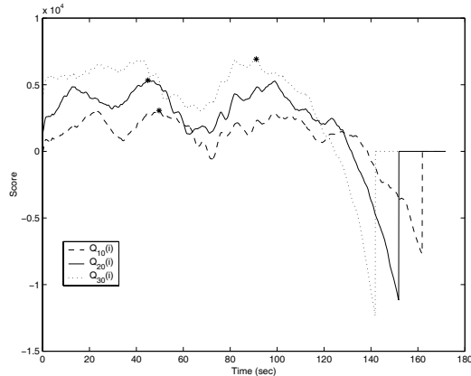
Figure 9: Summary scores, Q_L(i) , computed from the similarity matrix of Figure 7 for L = 10, 20 , and 30 seconds.
