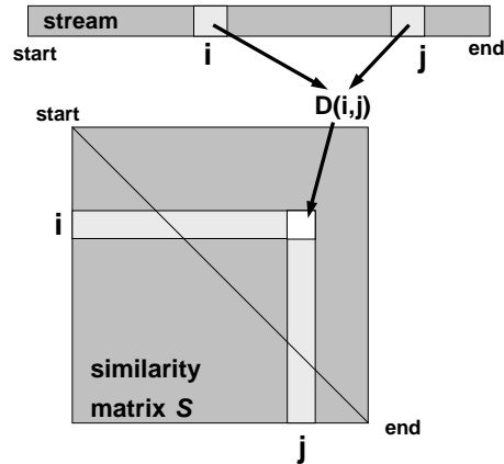
Figure 1: Embedding pairwise similarity data in the similarity matrix.
